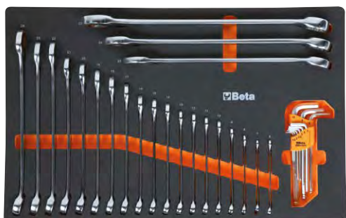
42C 6-7-8-9-10-11-12-13-14-15-16-17-18-19-20-21-22-23-24-27-30-32 mm 96BPC/SK9 1,5-2-2,5-3-4-5-6-8-10 mm
